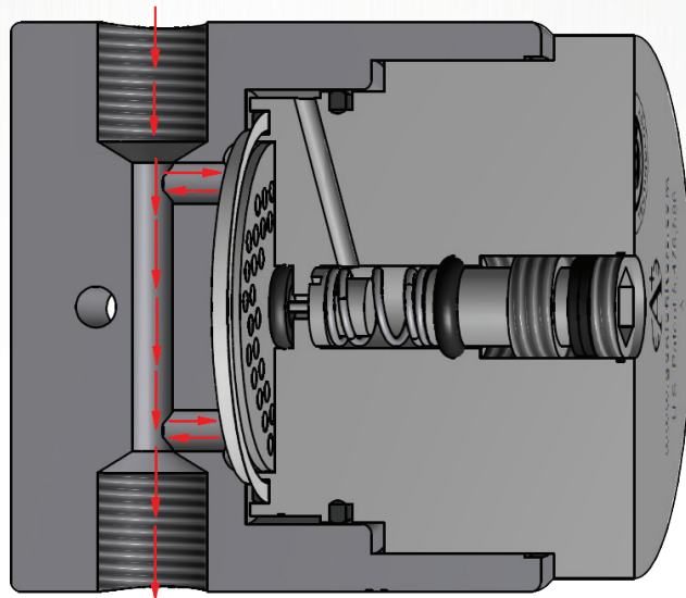
LIQUID BLOCK™ CLOSED
