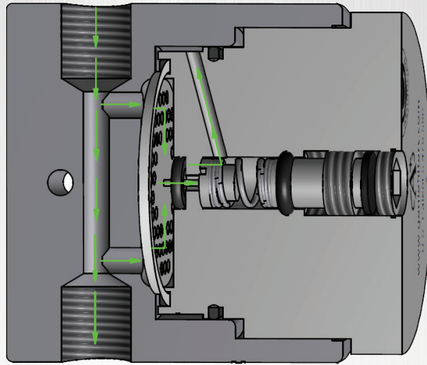
LIQUID BLOCK™ OPEN
